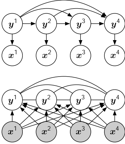
Figure 1: Graphical model showing the factorization of our noisy channel model where \mathbf{y}^i indicates the i th target language sentence and \mathbf{x}^i indicates the i th source language sentence. In the prior (top) the target sentences (the \mathbf{y}^i 's) only influence the corresponding source sentence and therefore can be learned and modeled independently, but at test time (bottom), when the target is not observed, each \mathbf{y}^i depends on every \mathbf{x}^i .
